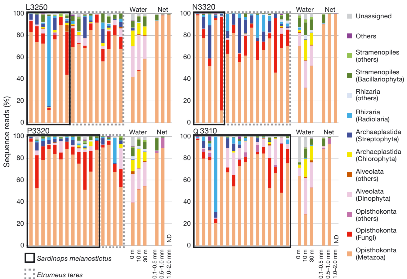
Fig. 2. Taxonomic percentages of sequence reads in Eukaryota, represented by the gut contents, microplankton (water), and mesoplankton (net) at each sampling station. 'Others' include Amoebozoa, Excavata, and Hacrobia. ND: no data
